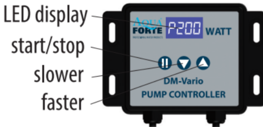
Figure 3. LED Display
